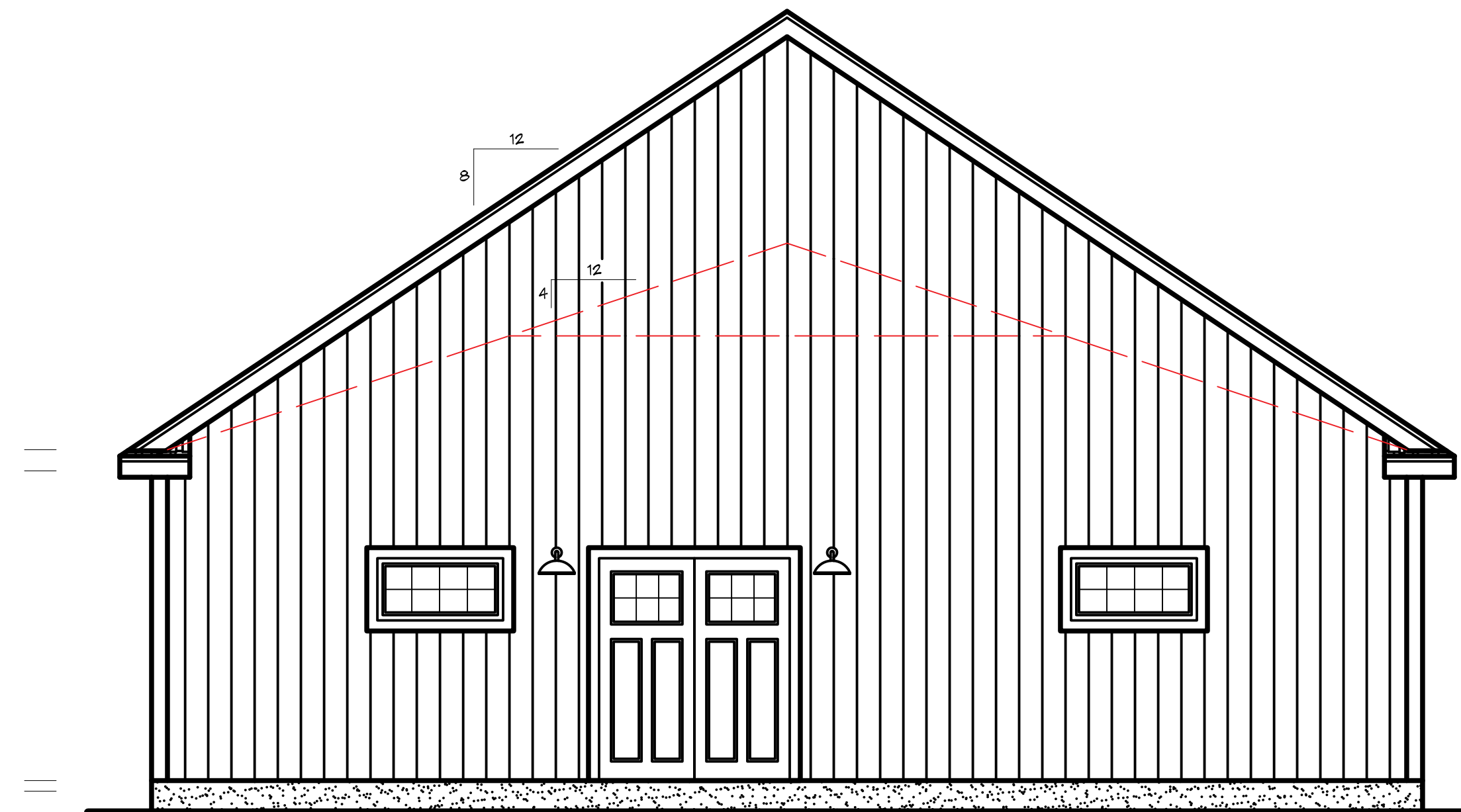
LEFT ELEVATION
